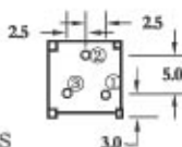
WI112-3(3386P)
