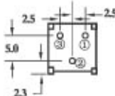
WI112-4(3386T)
